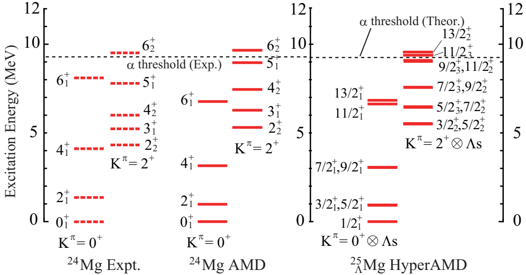
FIG. 3: Energy level schemes calculated by HyperAMD[14].(Left) Experimental and calculated level schemes of ^{24}\text{Mg} . (Right) A predicted level scheme of ^{25}_\Lambda\text{Mg} where a \Lambda is in s orbit.
