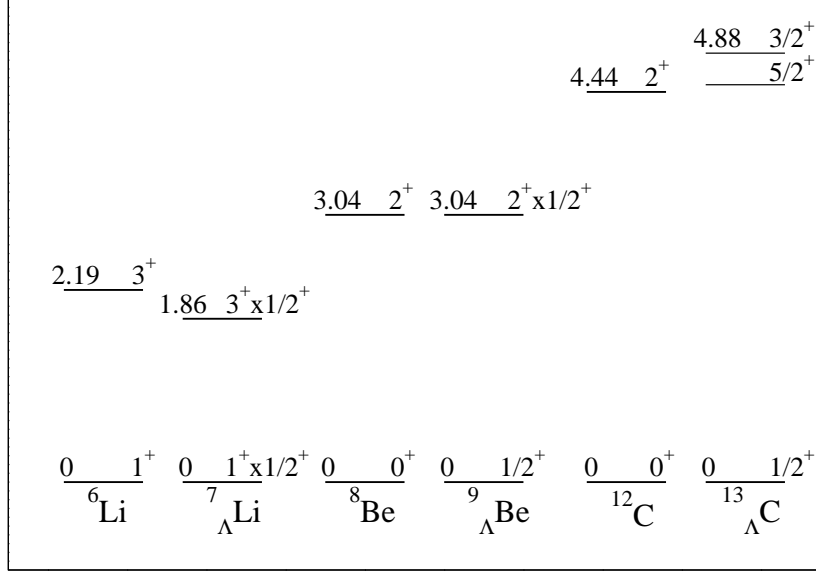
FIG. 1: The experimental low-lying spectra for {}^6\text{Li} , {}^7_{\Lambda}\text{Li} , {}^8\text{Be} , {}^9_{\Lambda}\text{Be} , {}^{12}\text{C} , and {}^{13}_{\Lambda}\text{C} nuclei. The energies are denoted in the units of MeV. The energies for the 1^+ \otimes 1/2^+ and 2^+ \otimes 1/2^+ levels of the {}^7_{\Lambda}\text{Li} nucleus are obtained by spin-averaging the observed level energies for the 1/2^+ (0 MeV) and the 3/2^+ (0.069 MeV) states, and the 5/2^+ (2.05 MeV) and the 7/2^+ (2.52 MeV) states [7], respectively. The energy for the 2^+ \otimes 1/2^+ level of the {}^9_{\Lambda}\text{Be} is the spin averaged energy between the 5/2^+ (3.02 MeV) and 3/2^+ (3.06 MeV) states [8]. In the {}^{13}_{\Lambda}\text{C} nucleus, only the energy for the 3/2^+ state has been measured [9], while the energy for the 5/2^+ state is expected to be lower than the energy of the 3/2^+ state by at most 0.36 MeV [10].
